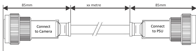
Illustration of a CA-JCMX-PT-XX Pre-Terminated Cable
