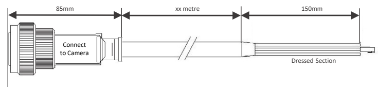
Illustration of a CA-JCMX-XX Not Pre-Terminated Cable (Dressed)
